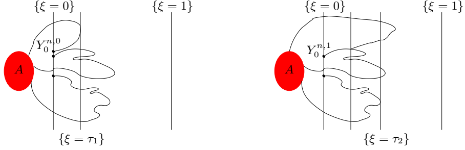
Figure 2: The first two steps of AMS with N = 3 trajectories.
