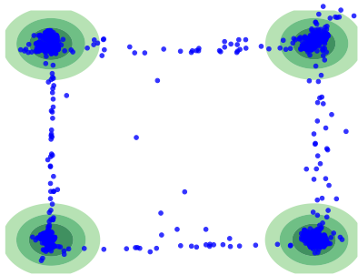
(a) True distribution \mu^* (mixture of K = 4 bivariate Gaussian densities, green circles) and 2000 data points sampled from the generator \mu_{\bar{g}} (blue dots).
