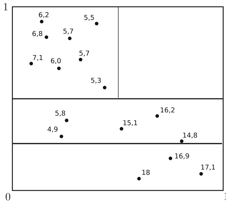
Fig. 1 A centered tree at level 2
