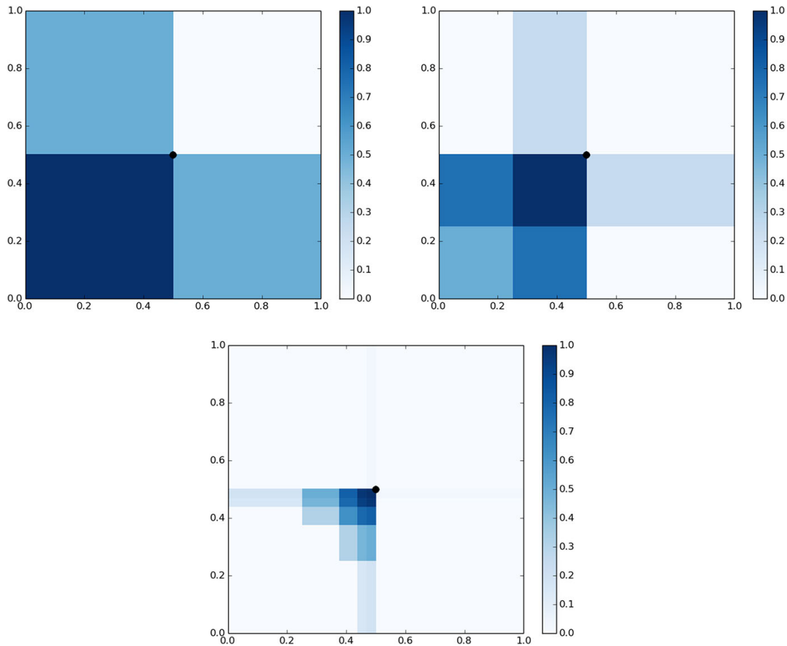
Fig. 3 Representations of f_1 , f_2 and f_5 in [0, 1]^2
