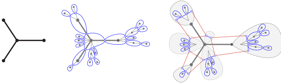
FIGURE 10. The discrete looptree \text{Loop}(T_n^{(S)}) can be constructed from the collection of modified looptrees (\widetilde{\text{Loop}}(\underline{P}_i^n))_i by identifying vertices connected by dashed edges.
