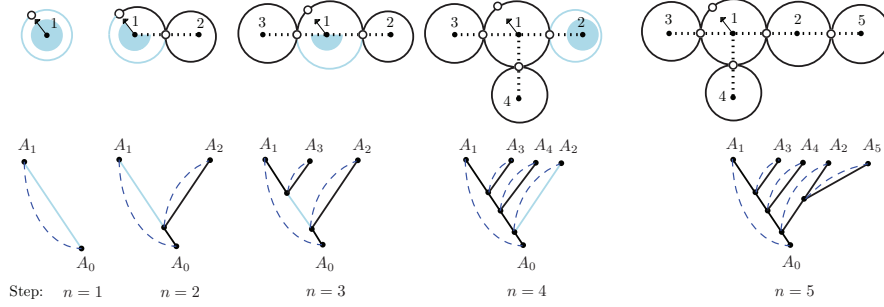
FIGURE 6. Illustration of the proof of Proposition 10, where in addition the edges that are split have been coupled in such a way that \text{Loop}(T_n^{-\circ}) = \text{Glu}(\mathbf{B}_n) . The first line represents the evolution of (T_n^{-\circ}, \text{Loop}(T_n^{-\circ}))_{1 \leq n \leq 5} and the second the evolution of (\mathbf{B}_n, \text{Glu}(\mathbf{B}_n))_{1 \leq n \leq 5} . In the second line, the dashed lines represent the identifications that are made.
